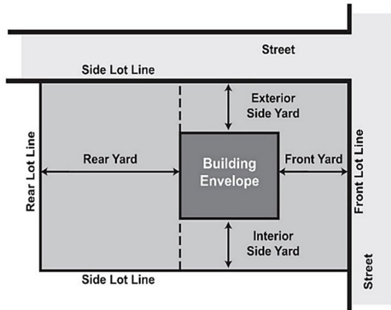
Figure 6.02.3, Building Envelope
